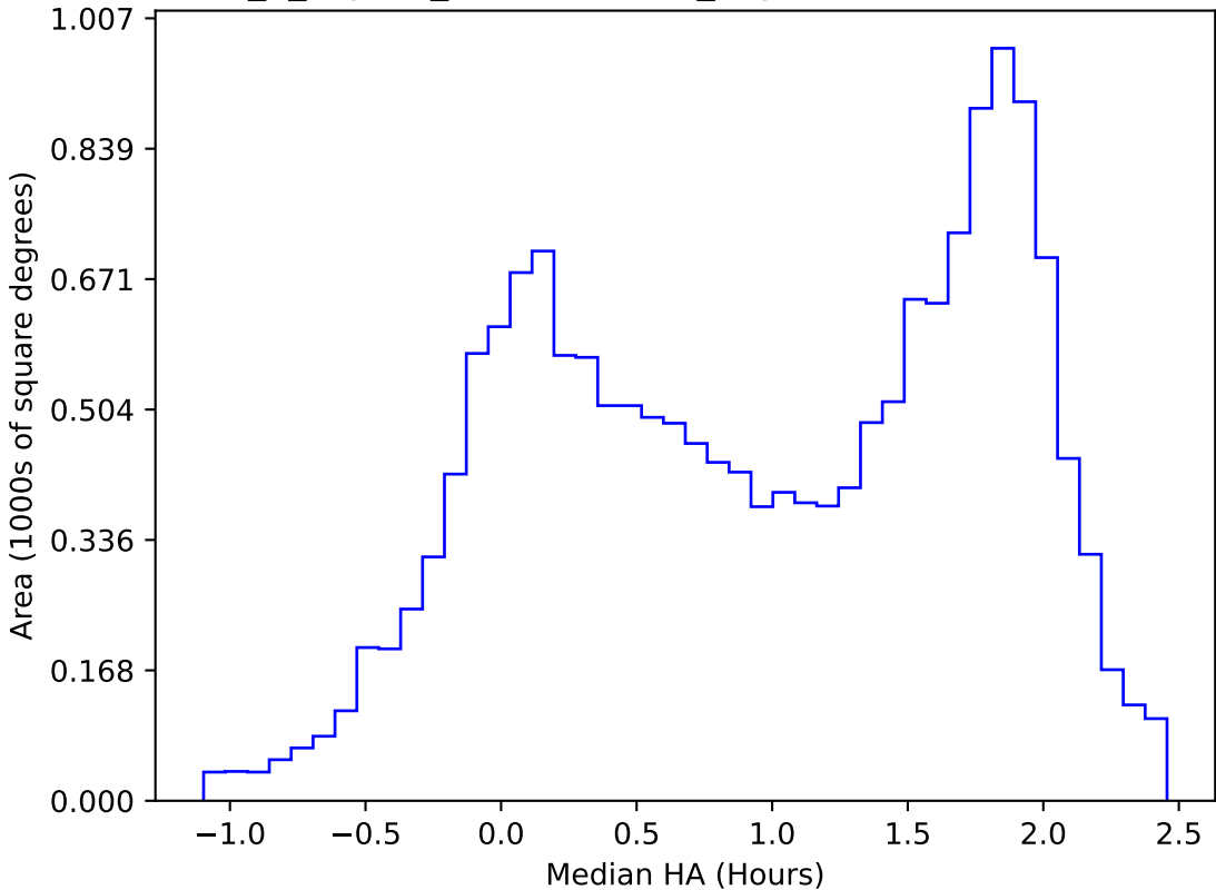
internal_u_expt30_nscale1.5v3.4_10yrs WFD u band: Median HA
