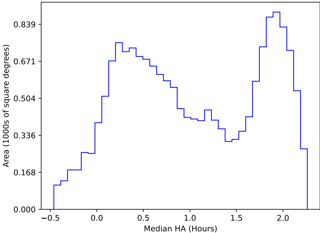
internal_u_expt30_nscale1.5v3.4_10yrs WFD i band: Median HA
