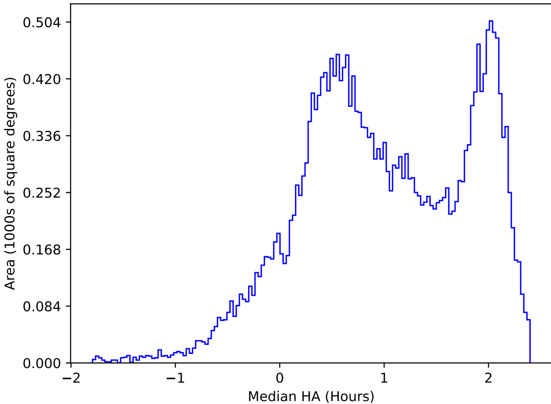
internal_u_expt30_nscale1.5v3.4_10yrs All sky z band: Median HA
