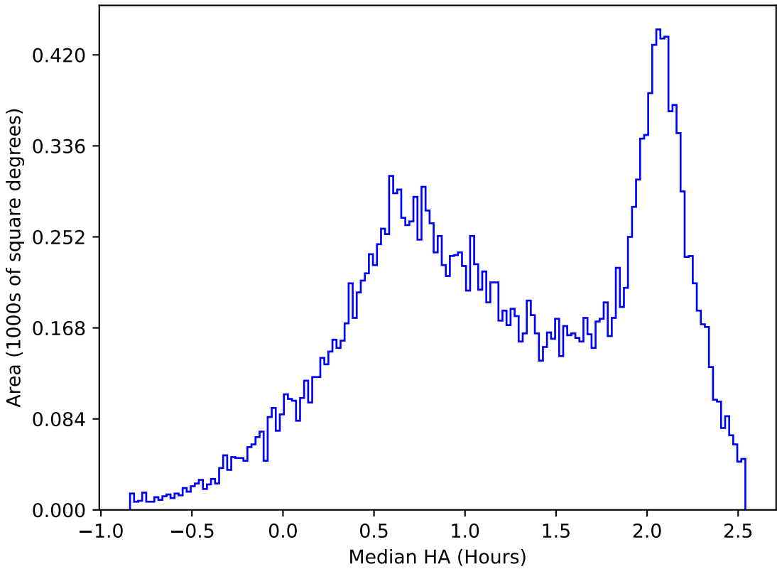
internal_u_expt30_nscale1.5v3.4_10yrs All sky y band: Median HA
