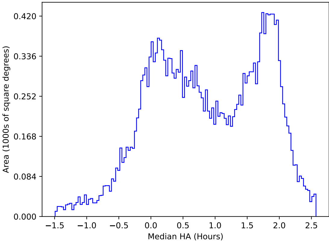
internal_u_expt30_nscale1.5v3.4_10yrs All sky u band: Median HA
