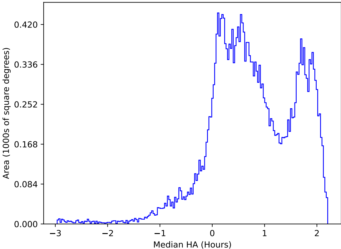
internal_u_expt30_nscale1.5v3.4_10yrs All sky r band: Median HA
