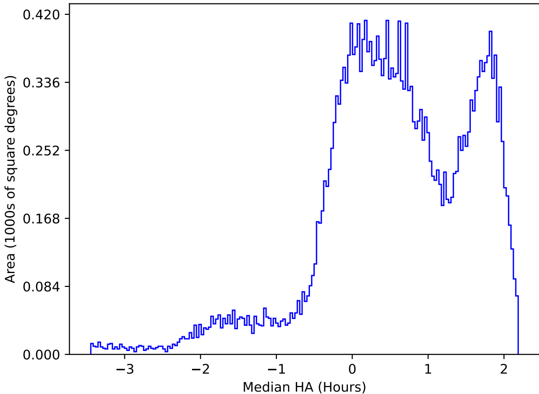
internal_u_expt30_nscale1.5v3.4_10yrs All sky g band: Median HA
