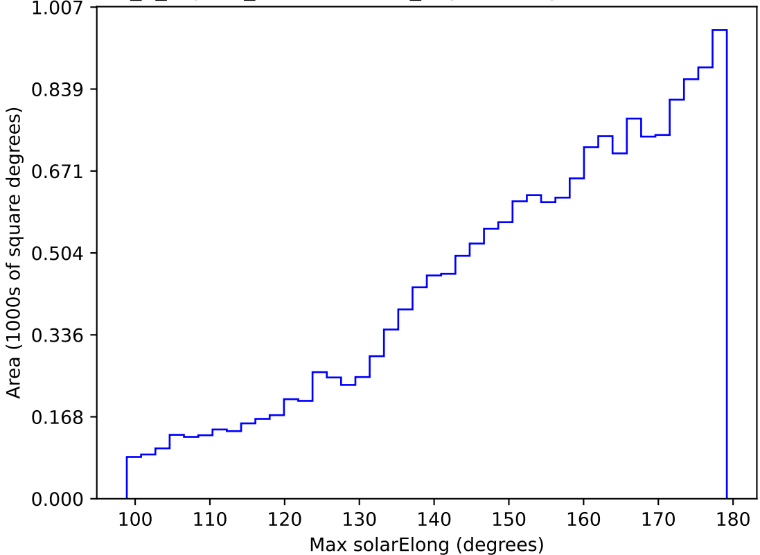
internal_u_expt30_nscale1.5v3.4_10yrs WFD y band: Max solarElong
