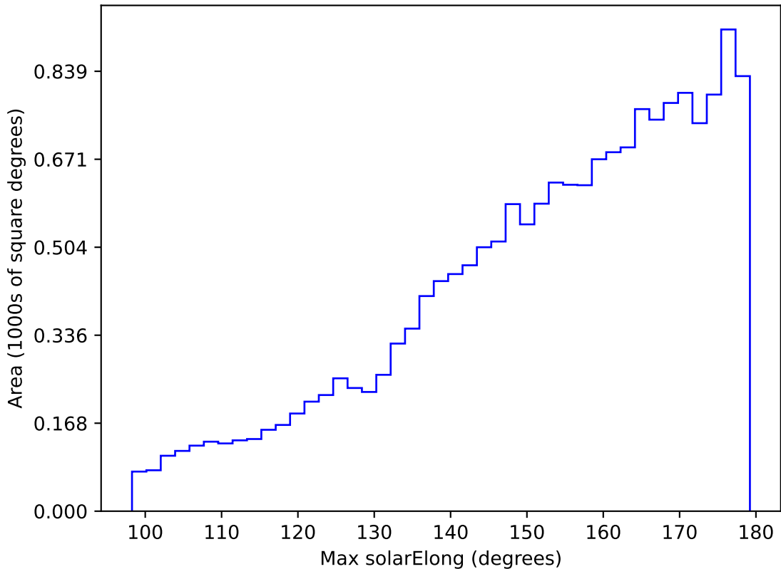
internal_u_expt30_nscale1.5v3.4_10yrs WFD u band: Max solarElong
