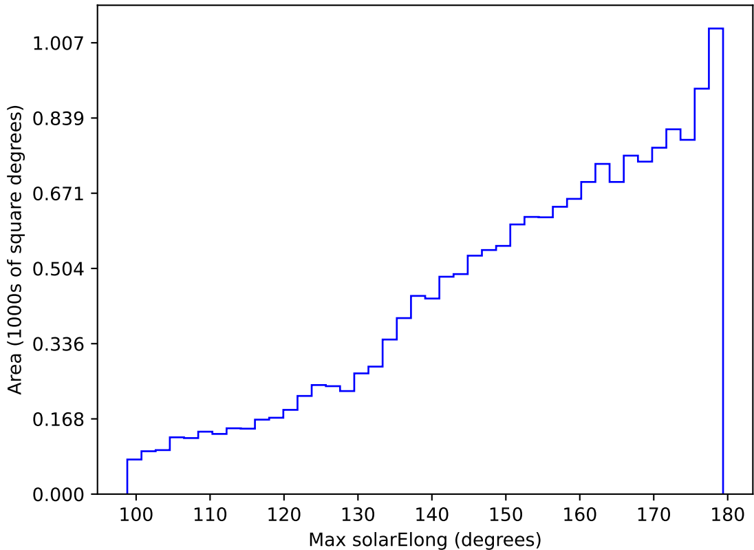
internal_u_expt30_nscale1.5v3.4_10yrs WFD r band: Max solarElong
