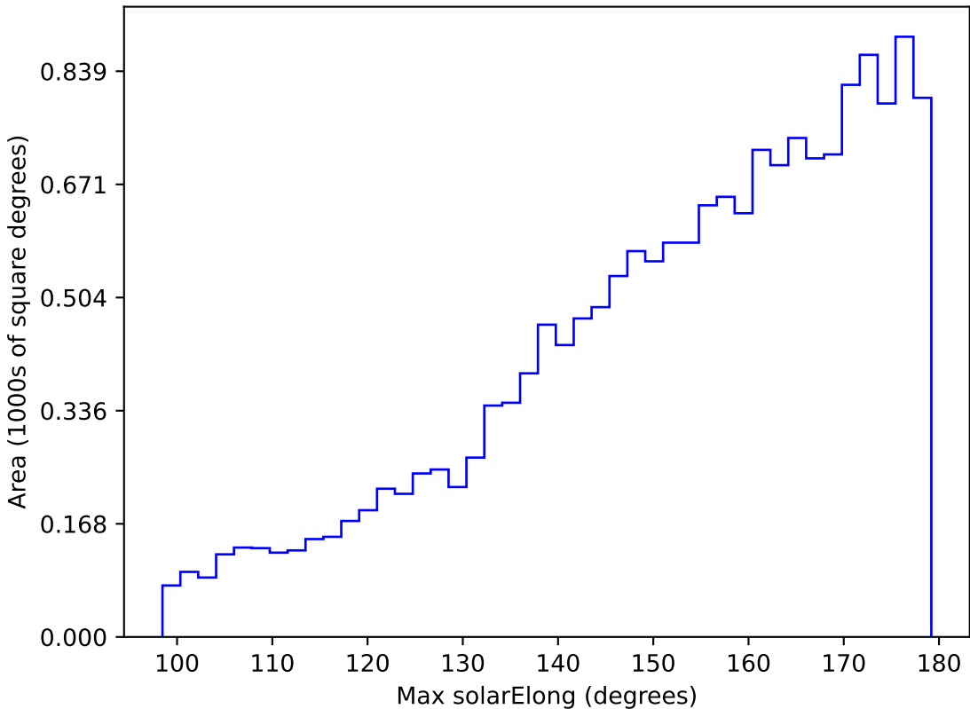
internal_u_expt30_nscale1.5v3.4_10yrs WFD g band: Max solarElong
