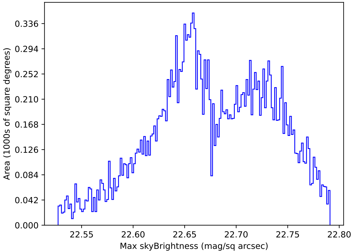
internal_u_expt30_nscale1.5v3.4_10yrs Yr 1 u band: Max skyBrightness
