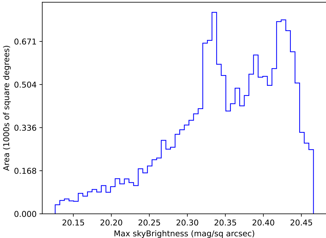
internal_u_expt30_nscale1.5v3.4_10yrs WFD i band: Max skyBrightness
