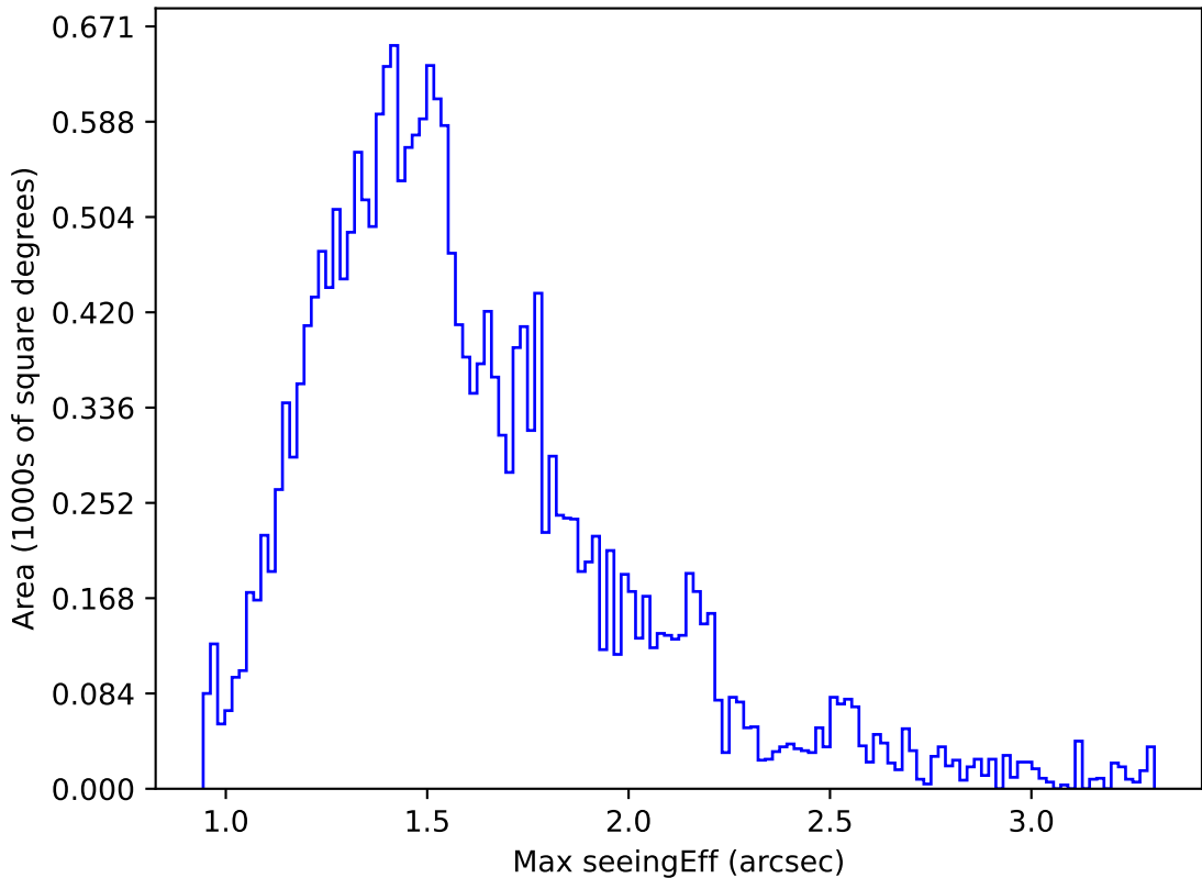
internal_u_expt30_nscale1.5v3.4_10yrs Yr 1 u band: Max seeingEff
