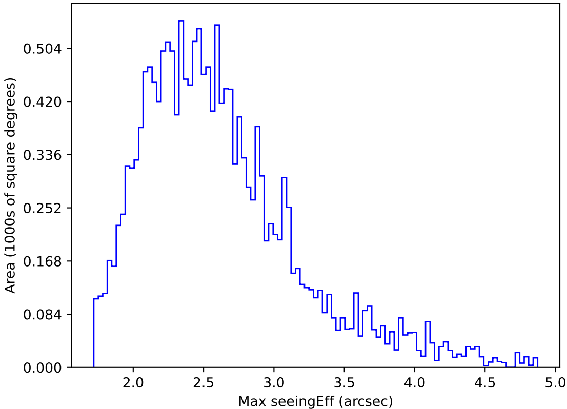
internal_u_expt30_nscale1.5v3.4_10yrs WFD z band: Max seeingEff
