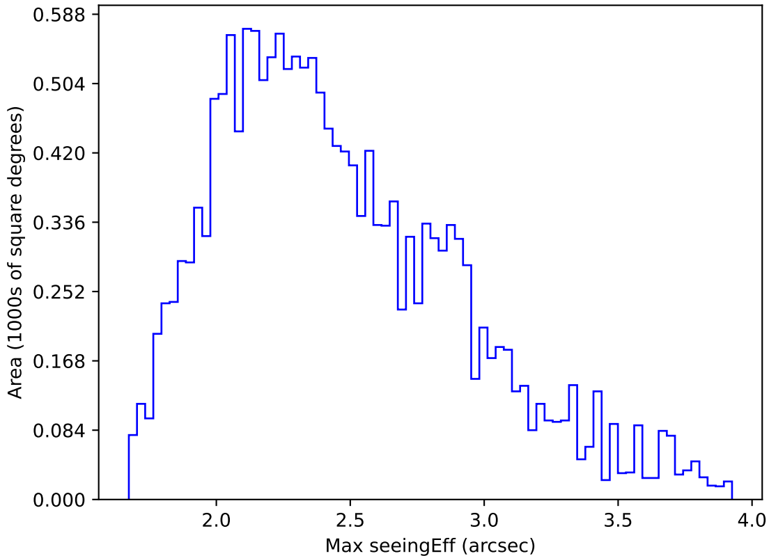
internal_u_expt30_nscale1.5v3.4_10yrs WFD g band: Max seeingEff
