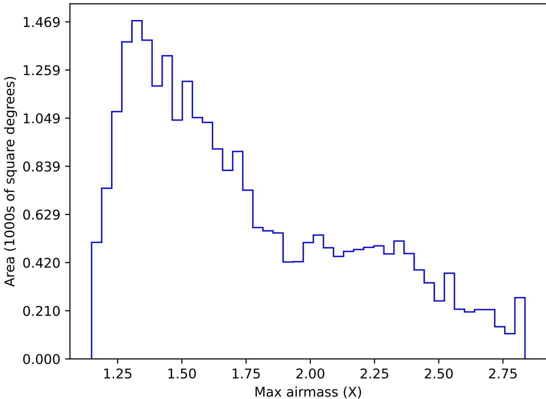
internal_u_expt30_nscale1.5v3.4_10yrs Yr 1 z band: Max airmass
