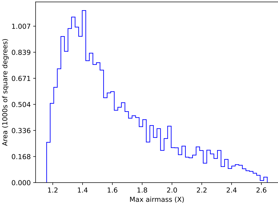
internal_u_expt30_nscale1.5v3.4_10yrs Yr 1 y band: Max airmass
