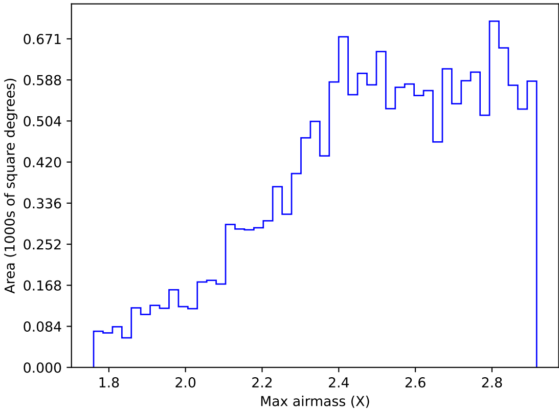
internal_u_expt30_nscale1.5v3.4_10yrs WFD z band: Max airmass
