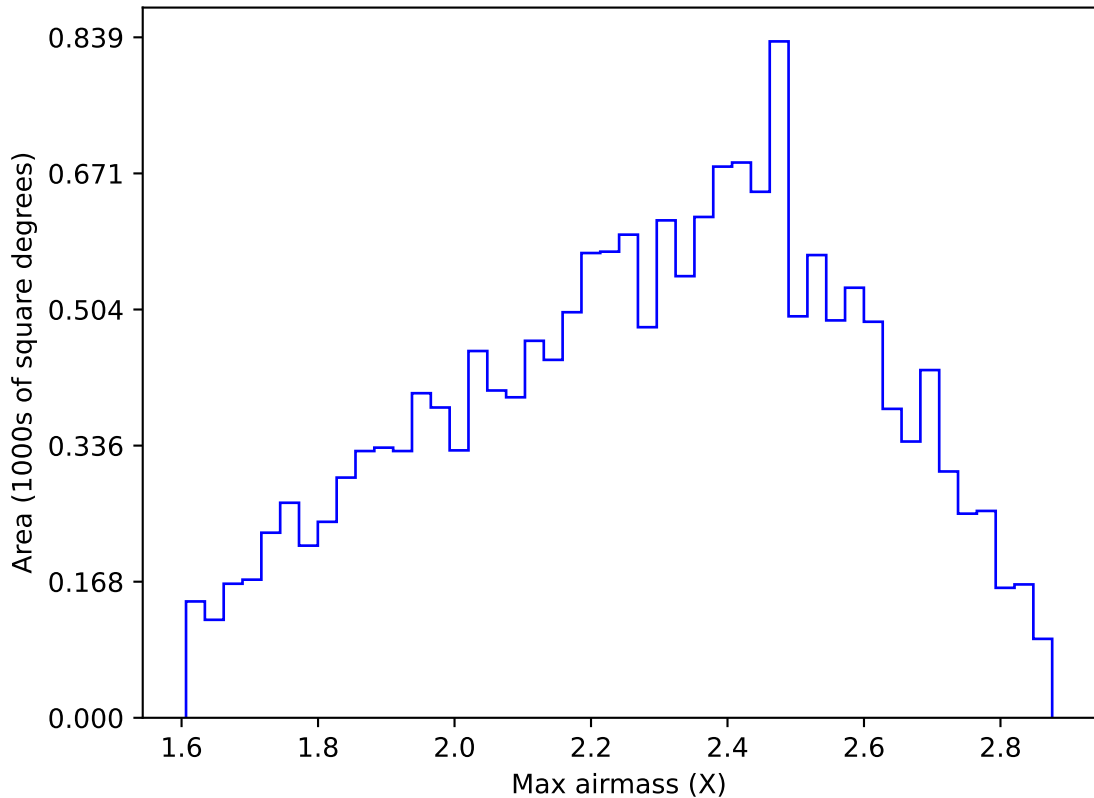
internal_u_expt30_nscale1.5v3.4_10yrs WFD y band: Max airmass
