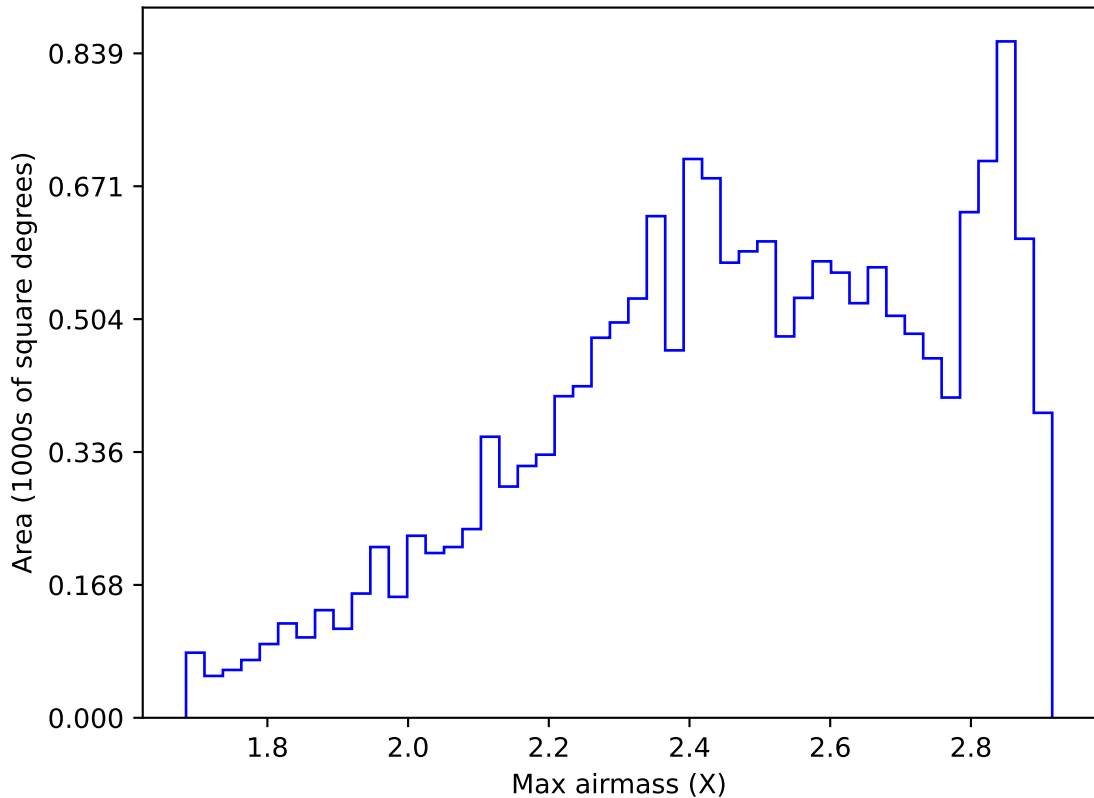
internal_u_expt30_nscale1.5v3.4_10yrs WFD i band: Max airmass
