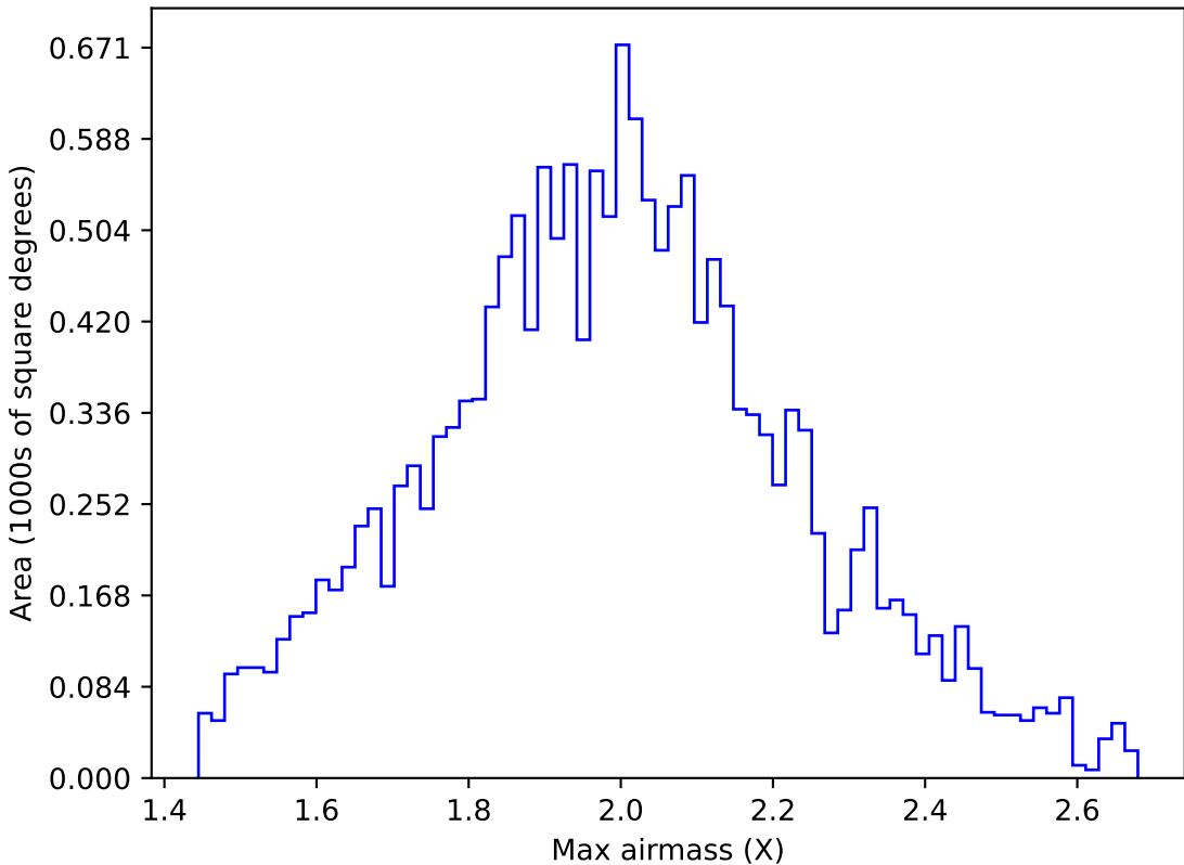
internal_u_expt30_nscale1.5v3.4_10yrs WFD g band: Max airmass
