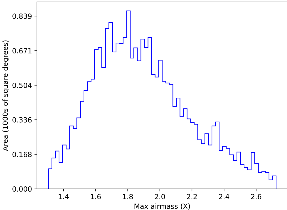
internal_u_expt30_nscale1.5v3.4_10yrs All sky u band: Max airmass
