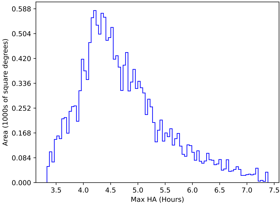
internal_u_expt30_nscale1.5v3.4_10yrs WFD y band: Max HA
