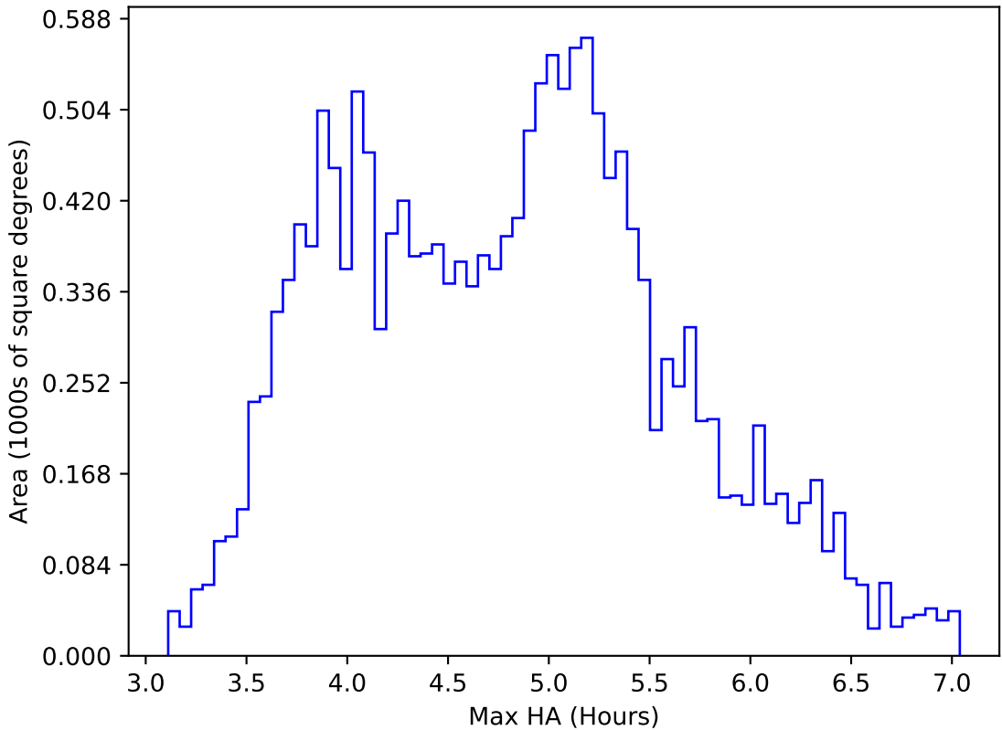
internal_u_expt30_nscale1.5v3.4_10yrs WFD i band: Max HA
