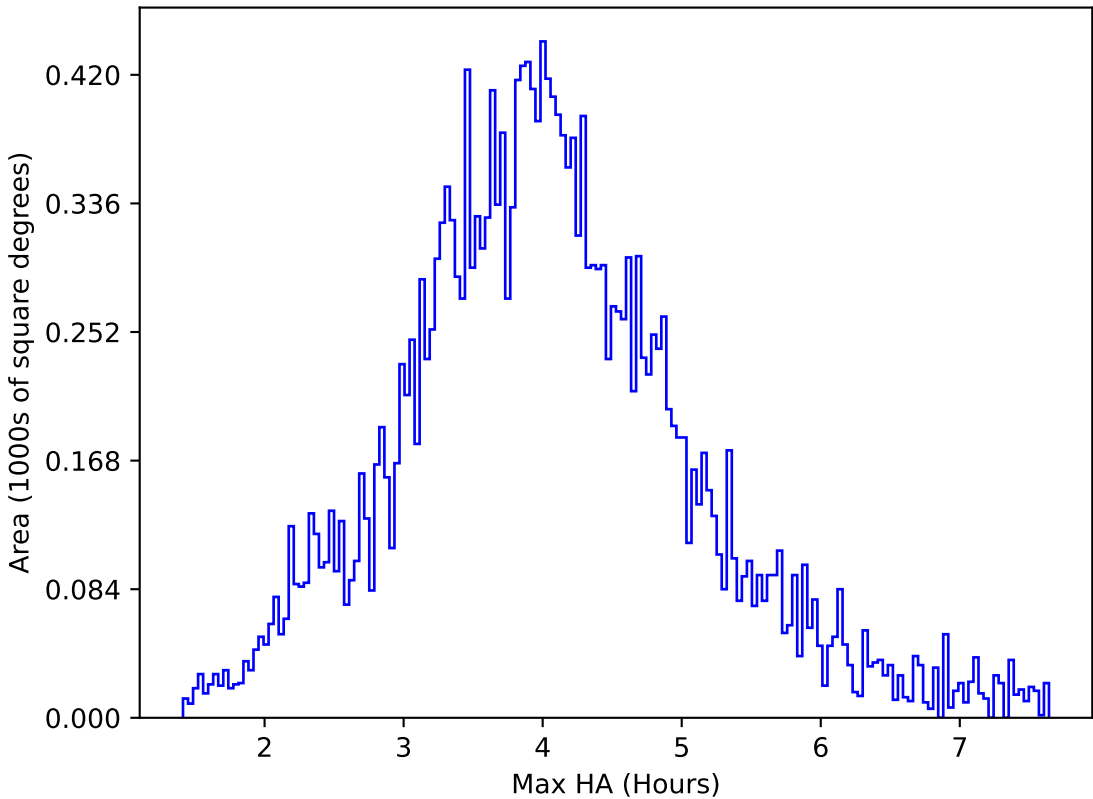
internal_u_expt30_nscale1.5v3.4_10yrs All sky u band: Max HA
