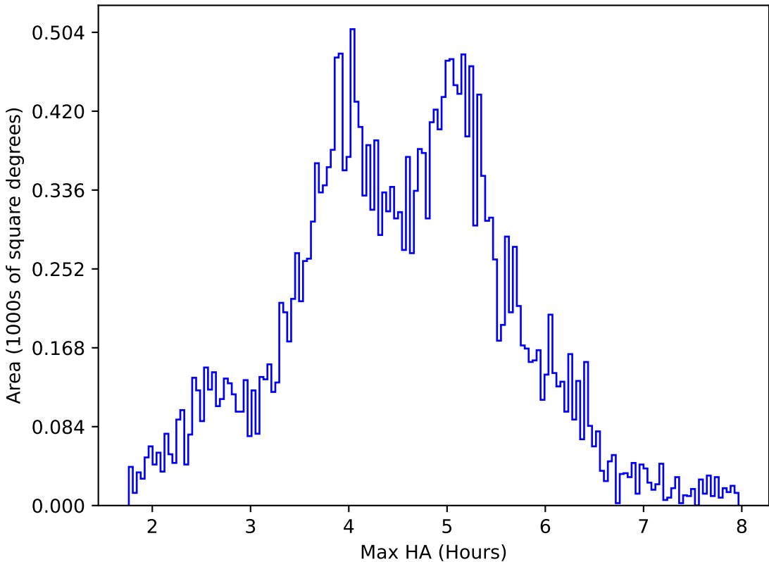
internal_u_expt30_nscale1.5v3.4_10yrs All sky i band: Max HA
