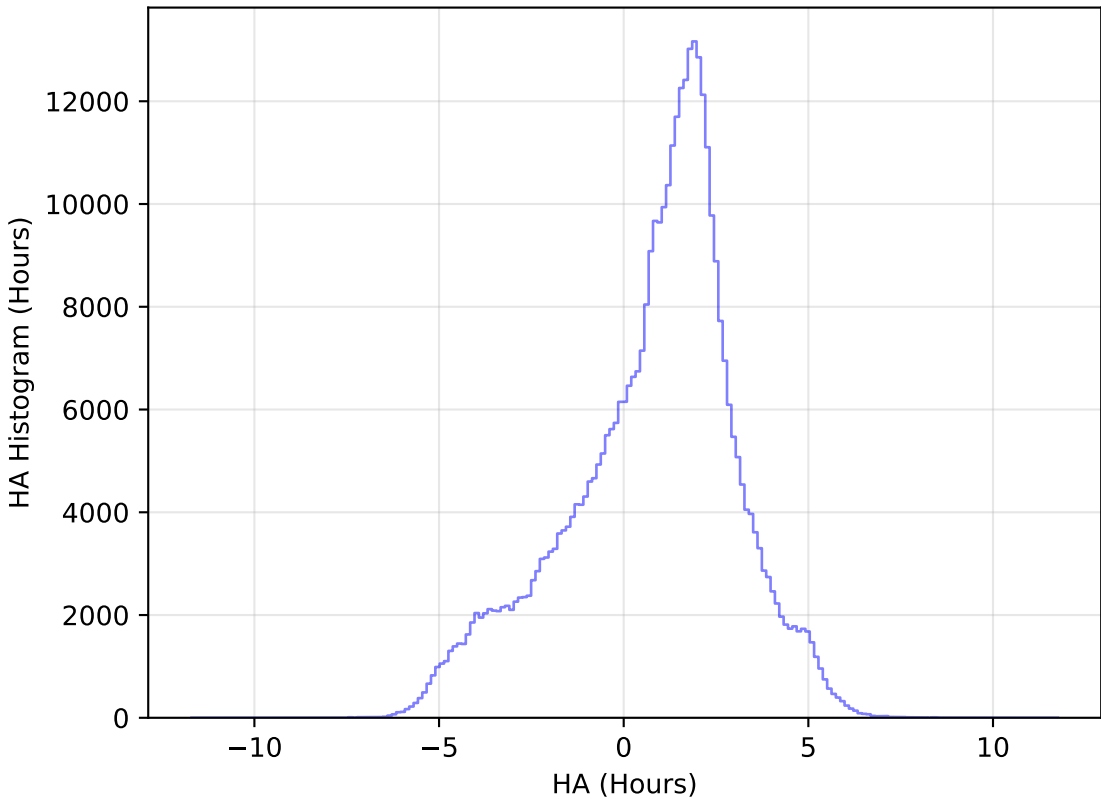
internal_u_expt30_nscale1.5v3.4_10yrs WFD z band: HA Histogram
