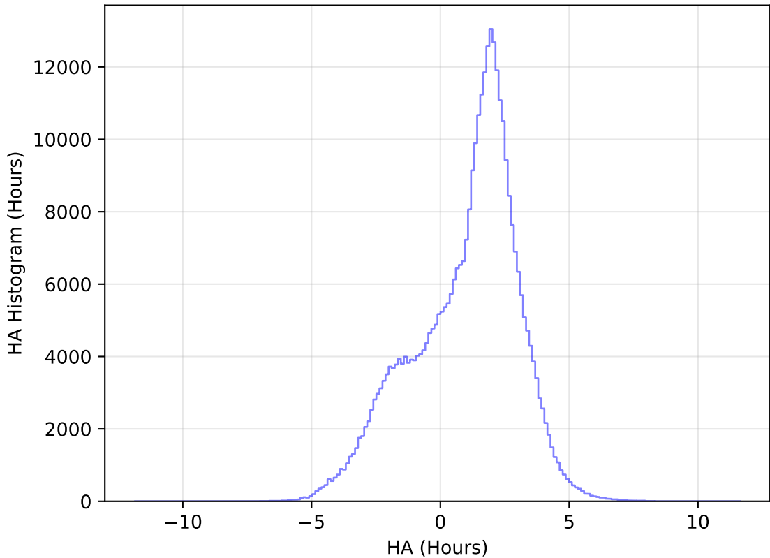
internal_u_expt30_nscale1.5v3.4_10yrs WFD y band: HA Histogram
