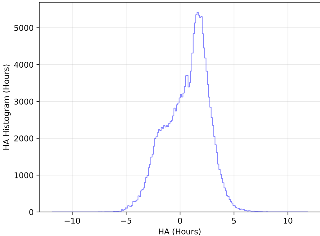
internal_u_expt30_nscale1.5v3.4_10yrs WFD u band: HA Histogram
