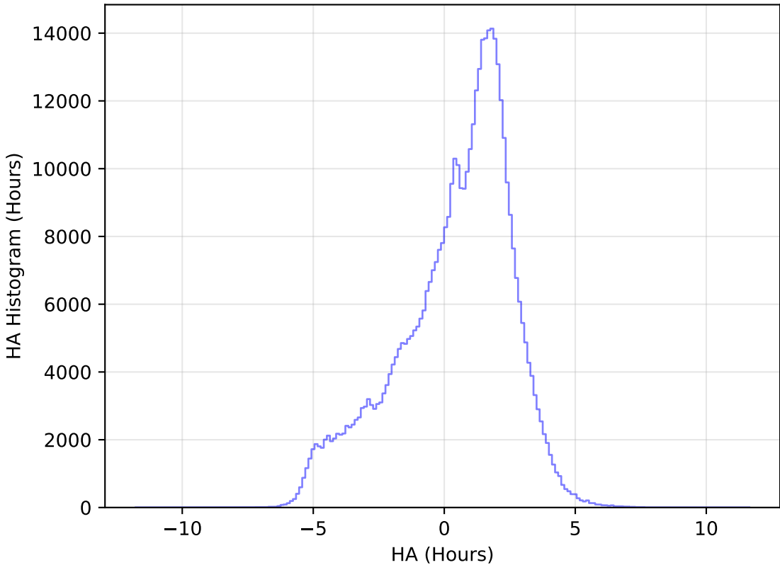
internal_u_expt30_nscale1.5v3.4_10yrs WFD r band: HA Histogram
