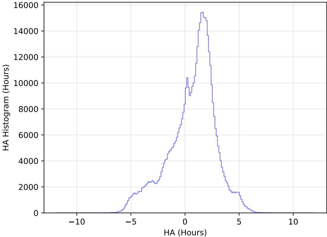
internal_u_expt30_nscale1.5v3.4_10yrs WFD i band: HA Histogram
