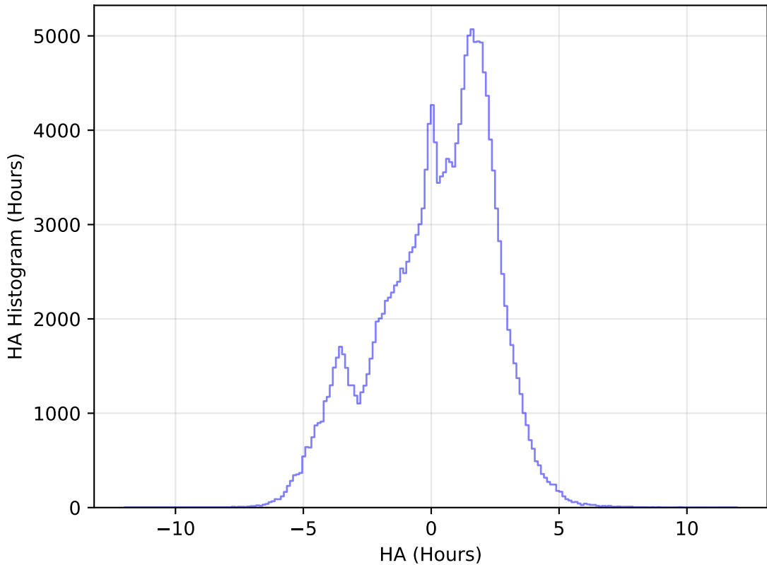
internal_u_expt30_nscale1.5v3.4_10yrs WFD g band: HA Histogram
