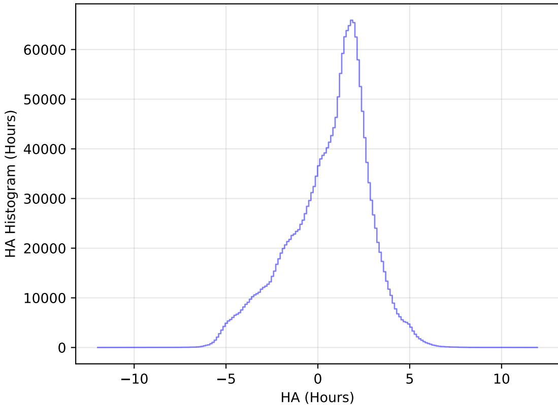
internal_u_expt30_nscale1.5v3.4_10yrs WFD all bands: HA Histogram
