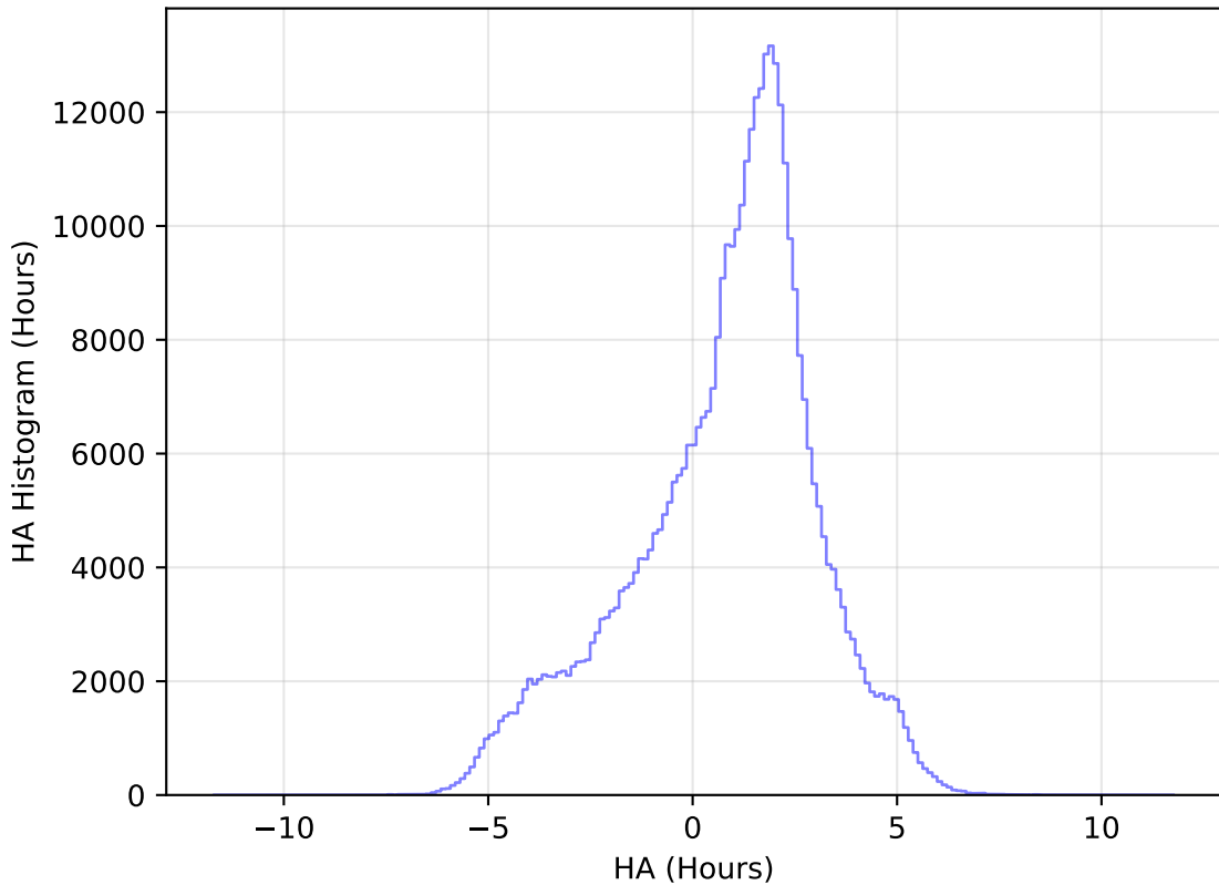
internal_u_expt30_nscale1.5v3.4_10yrs All sky z band: HA Histogram
