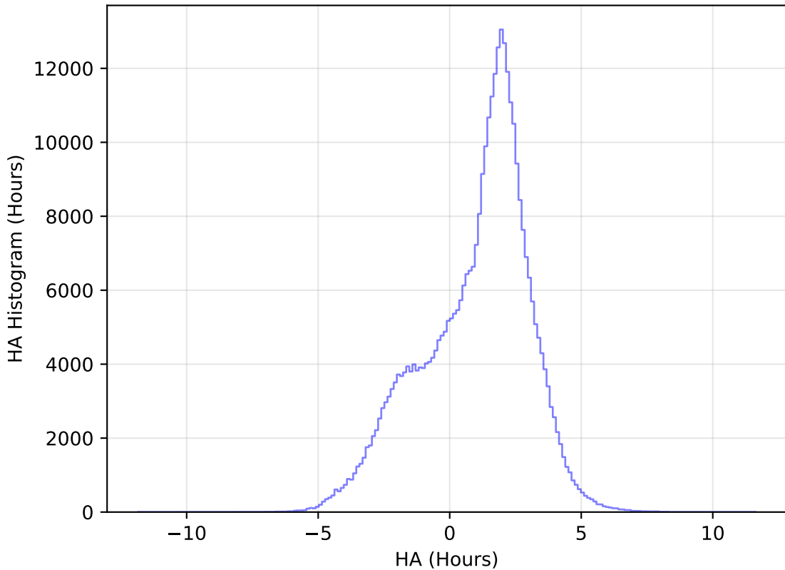
internal_u_expt30_nscale1.5v3.4_10yrs All sky y band: HA Histogram
