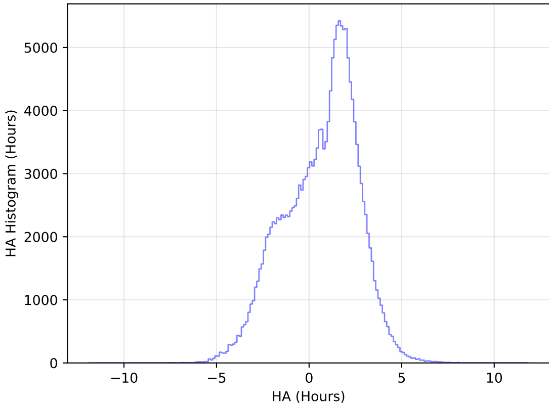
internal_u_expt30_nscale1.5v3.4_10yrs All sky u band: HA Histogram
