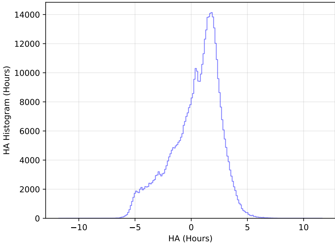
internal_u_expt30_nscale1.5v3.4_10yrs All sky r band: HA Histogram
