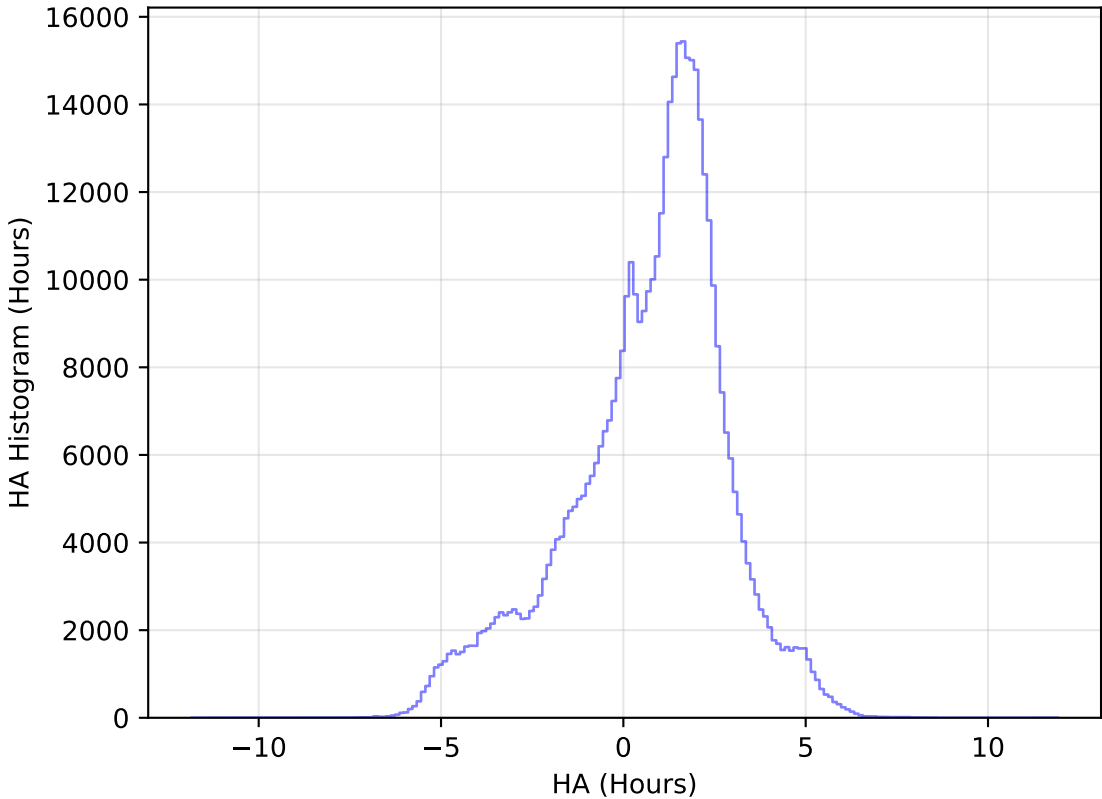
internal_u_expt30_nscale1.5v3.4_10yrs All sky i band: HA Histogram
