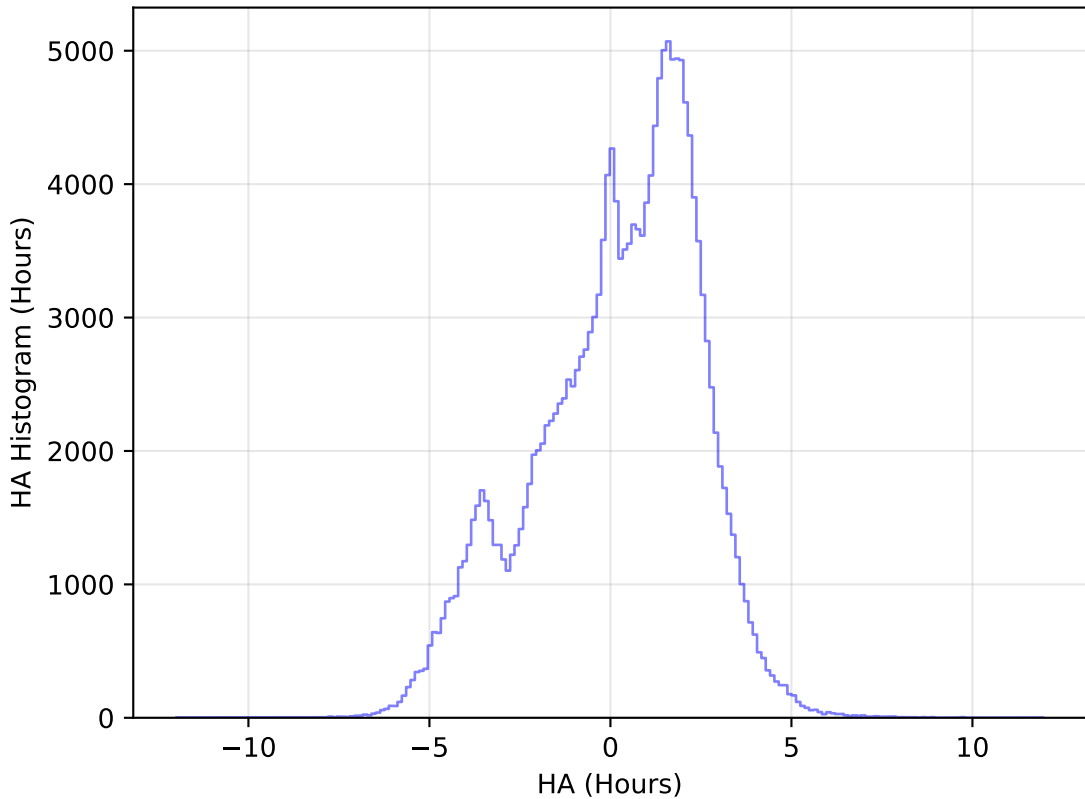
internal_u_expt30_nscale1.5v3.4_10yrs All sky g band: HA Histogram
