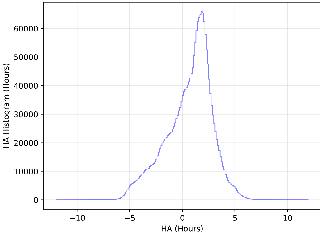
internal_u_expt30_nscale1.5v3.4_10yrs All sky all bands: HA Histogram
