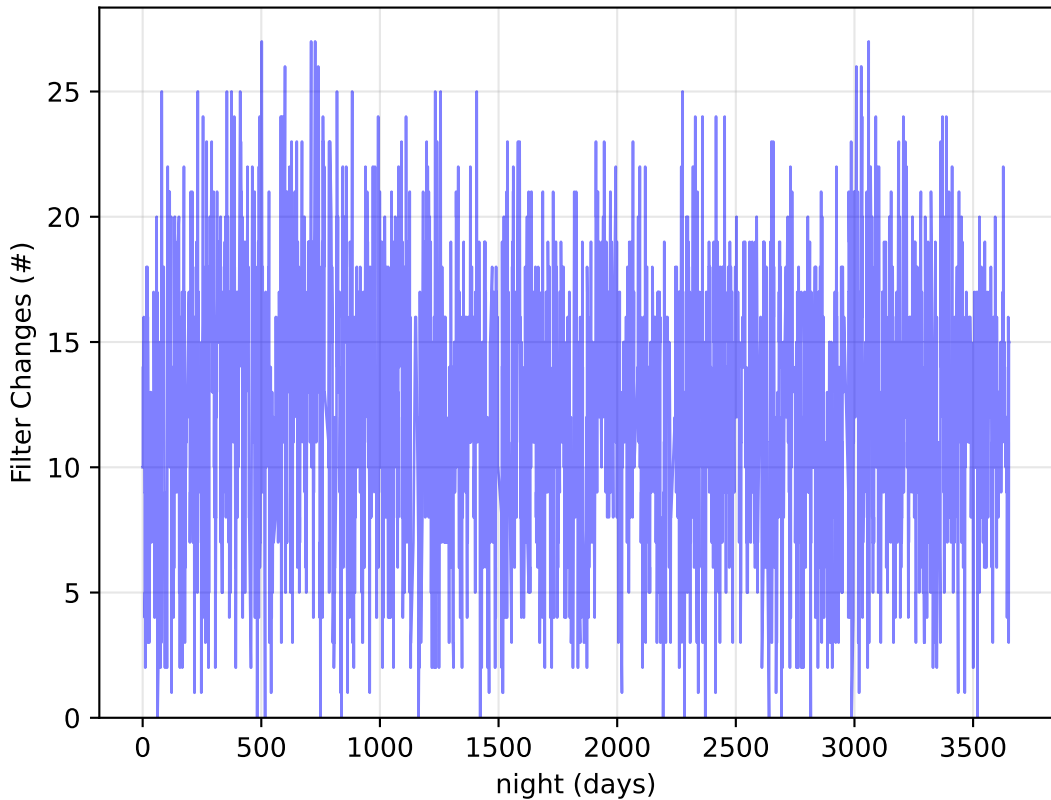
internal_u_expt30_nscale1.5v3.4_10yrs Per Night: Filter Changes
