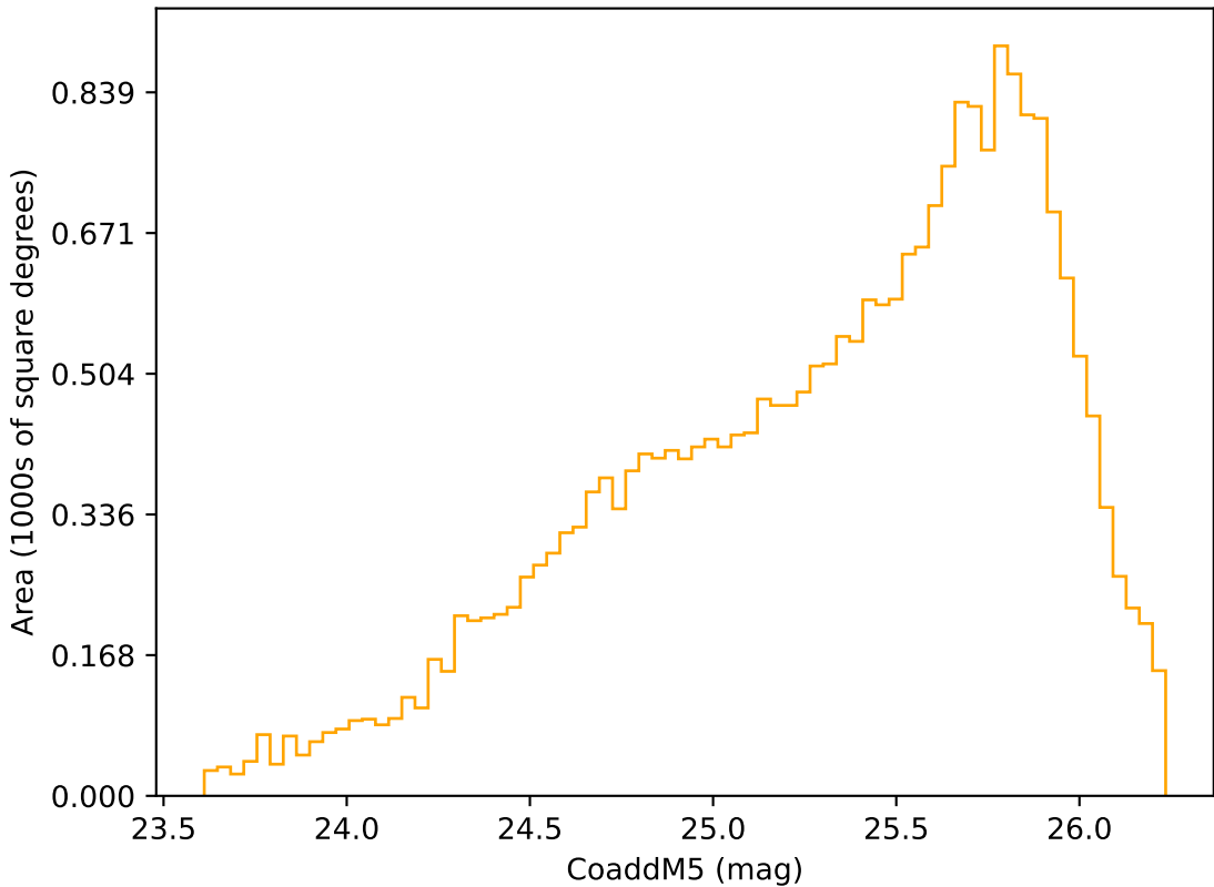
internal_u_expt30_nscale1.5v3.4_10yrs Yr 3-4 r band: CoaddM5
