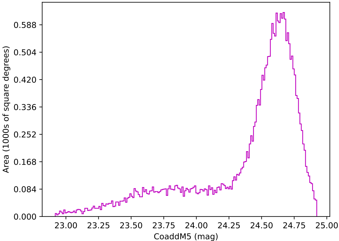
internal_u_expt30_nscale1.5v3.4_10yrs Yr 1 z band: CoaddM5
