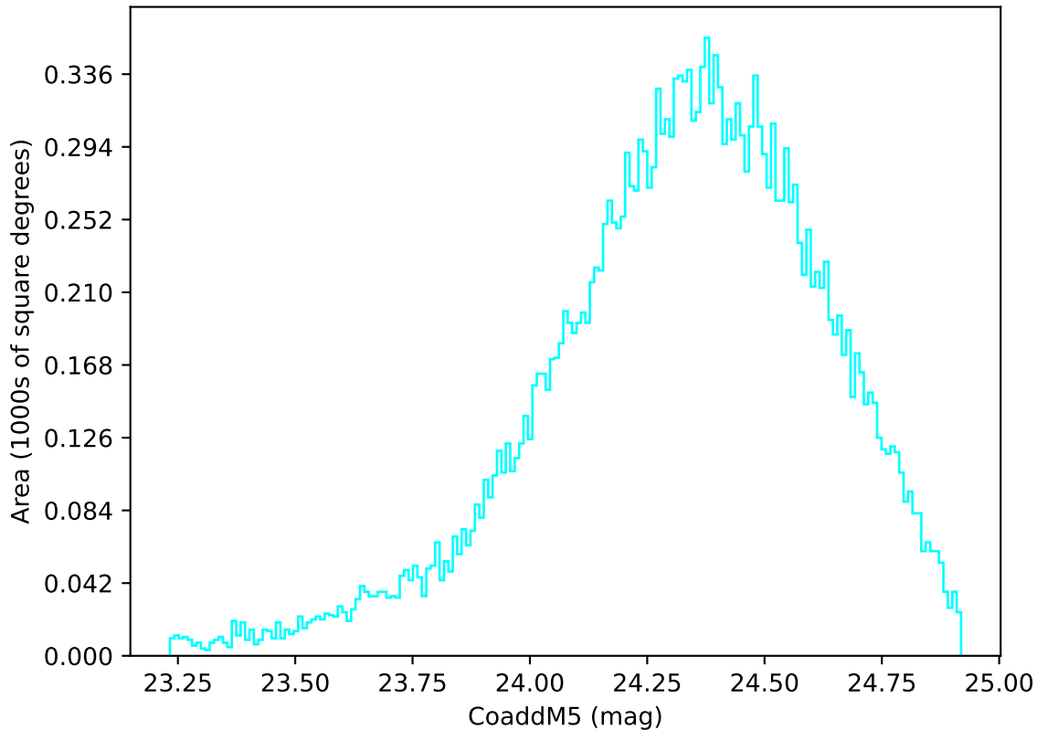
internal_u_expt30_nscale1.5v3.4_10yrs Yr 1 u band: CoaddM5
