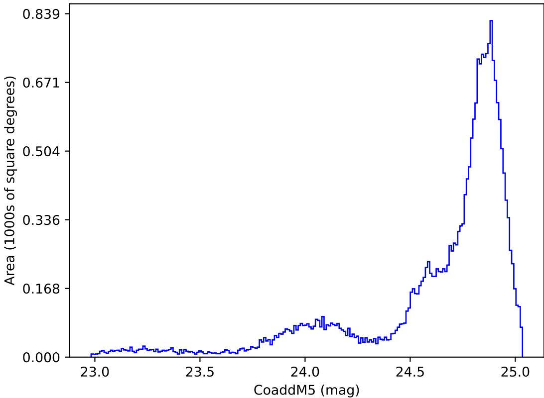
internal_u_expt30_nscale1.5v3.4_10yrs All sky y band: CoaddM5
