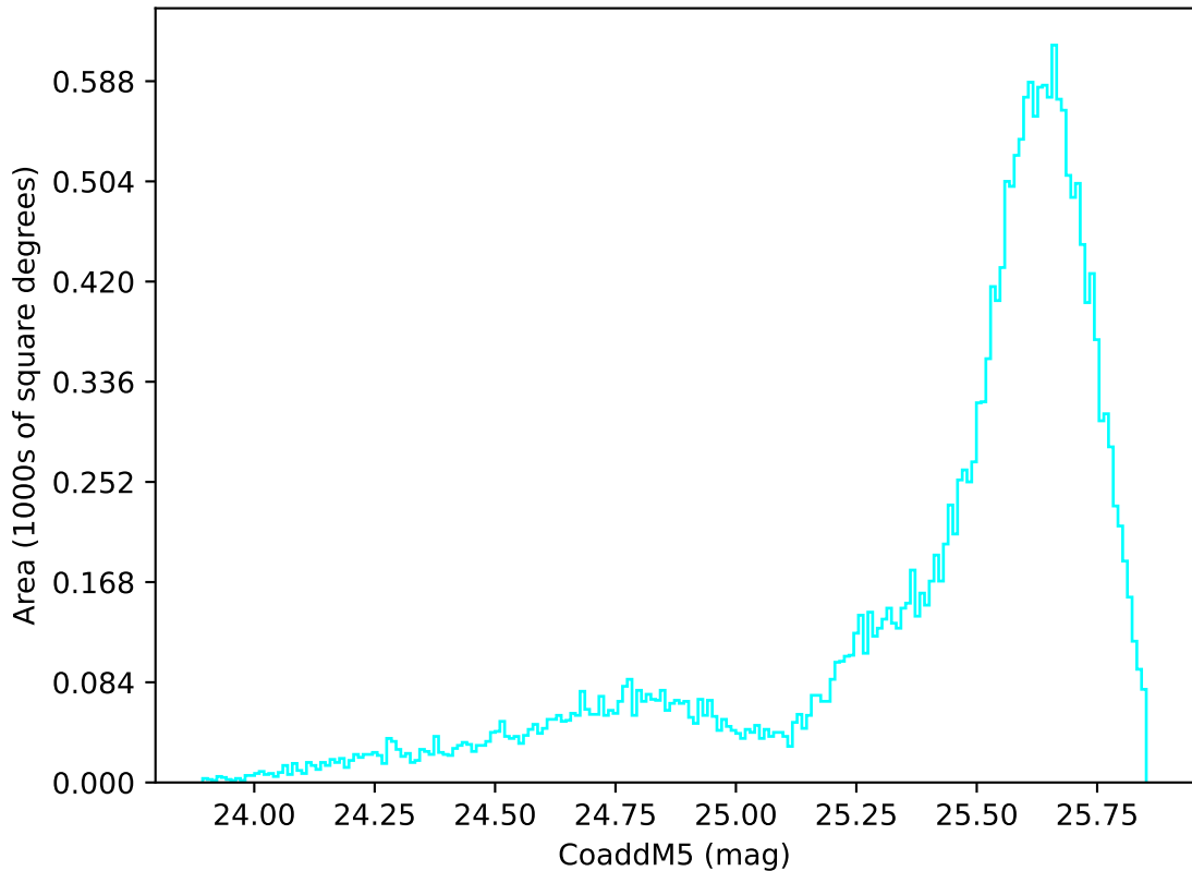
internal_u_expt30_nscale1.5v3.4_10yrs All sky u band: CoaddM5
