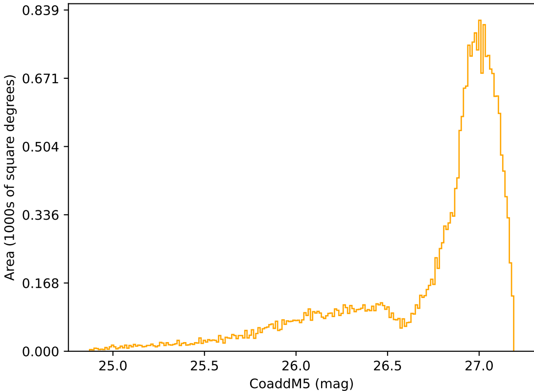
internal_u_expt30_nscale1.5v3.4_10yrs All sky r band: CoaddM5
