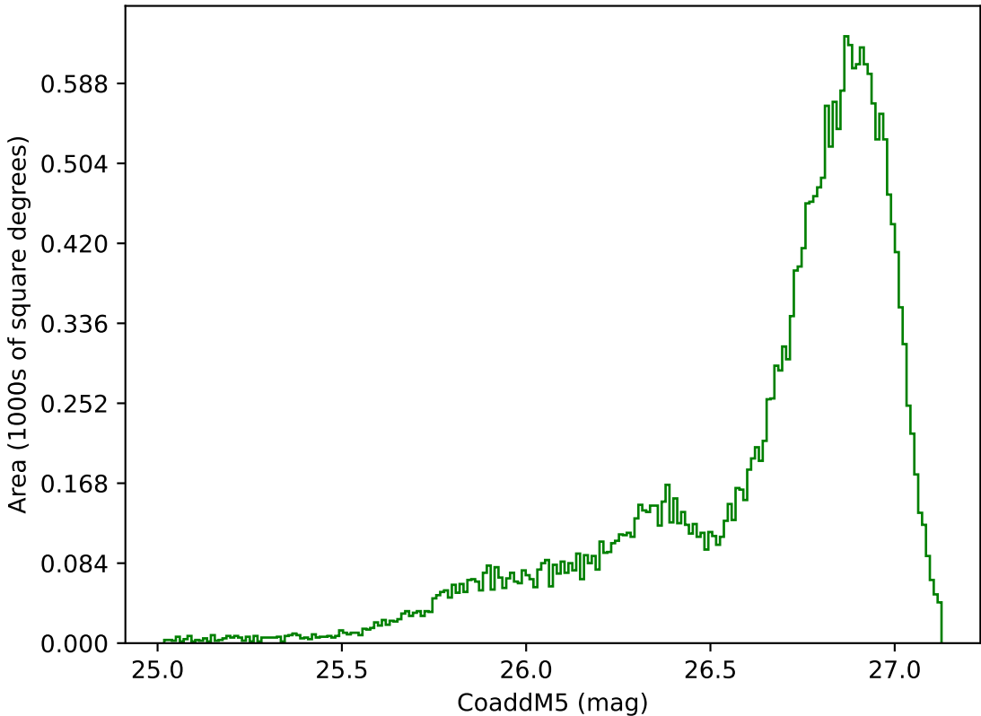
internal_u_expt30_nscale1.5v3.4_10yrs All sky g band: CoaddM5
