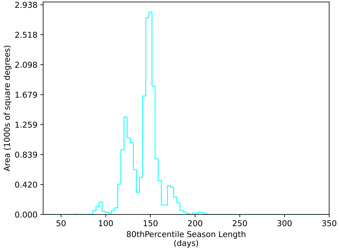
internal_u_expt30_nscale1.5v3.4_10yrs WFD u band: 80thPercentile Season Length
